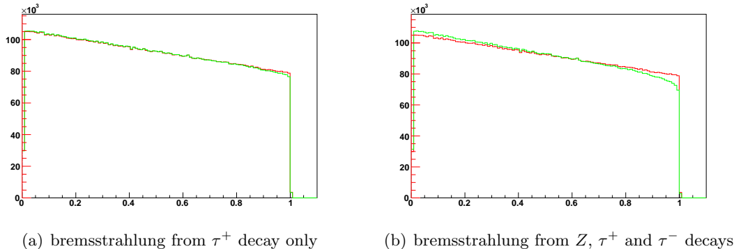
Figure 2: Bremsstrahlung effects for longitudinal spin observables for the cascade decay: Z \rightarrow \tau^+\tau^- , \tau^\pm \rightarrow \pi^\pm\nu . The \pi^+ energy spectrum in the Z rest-frame is shown. The red line is for bremsstrahlung switched off and green (light grey) when its effect is included. In the left plot, bremsstrahlung is in \tau^+ decay only. In the right plot, bremsstrahlung from Z and \tau^\pm decays is taken into account. These plots have been prepared using a custom UserTreeAnalysis of MC-TESTER. They can be recreated with the test located in the examples/testing/Ztautau directory, see examples/testing/README-plots for technical details. Results are consistent with Fig. 5 of Ref. [28].
