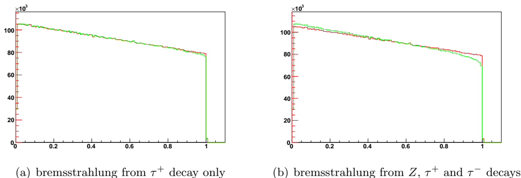
Figure 2: Bremsstrahlung effects for longitudinal spin observables for the cascade decay: Z \rightarrow \tau^+ \tau^- , \tau^\pm \rightarrow \pi^\pm \nu . \pi^+ energy spectrum in the Z rest-frame is shown. The red line is for bremsstrahlung switched off and green (light grey) when its effect is included. In the left plot, bremsstrahlung is in \tau^+ decay only. In the right plot, bremsstrahlung from Z and \tau^\pm decays is taken into account. These plots have been prepared using a custom UserTreeAnalysis of MC-TESTER . They can be recreated with the test located in the examples/testing/Ztautau directory, see examples/testing/README-plots for technical details. Results are consistent with Fig. 5 of Ref. [26].
