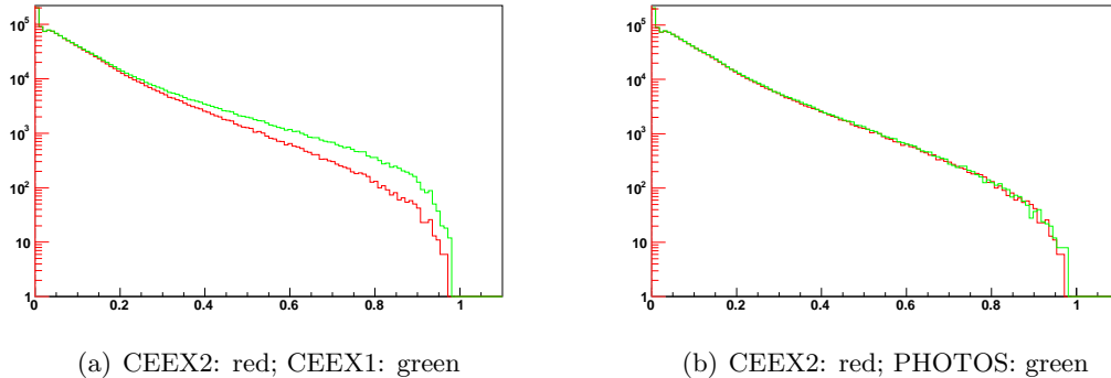
Figure 5: The spectrum of the \gamma\gamma invariant mass in Z \rightarrow \mu^+\mu^- decay. Events with two hard photons, both of energy above 1 GeV in the Z rest frame are taken. Comparisons are shown for CEEEX2 and CEEEX1 (left plot), and CEEEX2 and PHOTOS (right plot). The prediction from PHOTOS is clearly superior for applications aimed at the simulation of Higgs boson backgrounds. In the case of solutions based on YFS exponentiation, the second order matrix element must be taken into account. Fig. 5(b) was obtained from our example, examples/testing/Zmumu , after adaptation of the center-of-mass energy (91.17 GeV) and test energy threshold (1 GeV). Samples of 100 million events were used. See examples/testing/README-plots for technical details. Reference ROOT files for KKMC CEEEX samples are, however, created outside of the distribution.
